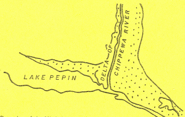
Damming of the Mississippi River by the Chippewa River to form Lake Pepin.
