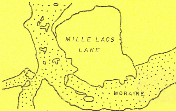
Moraine-dam lake: Mille Lacs Lake and Mille Lacs moraine.
