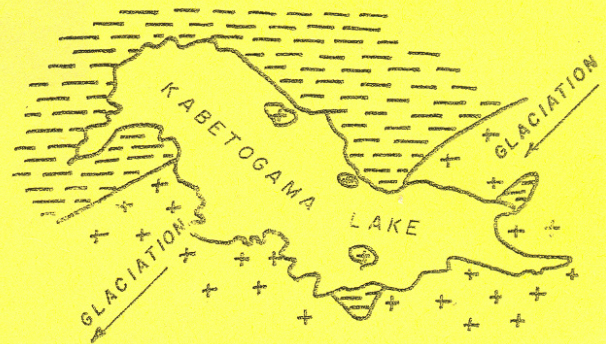
Lake in bedrock basin not related to preglacial valleys.
