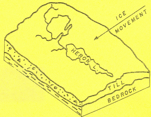
Lake in basin produced by irregular deposition of till: Heron Lake in northwestern Jackson County.
