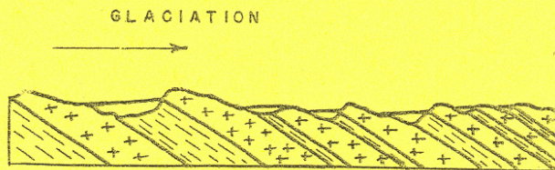
Lake basins in bedrock valleys in eroded slate.
