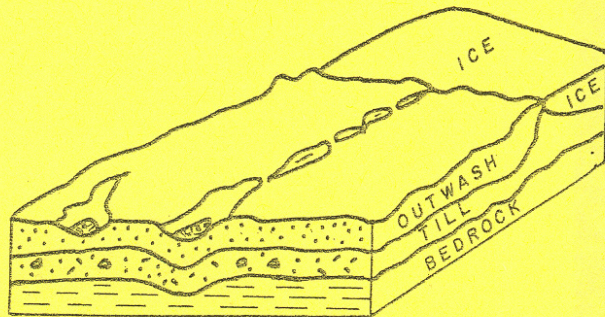
Lakes in ice-block basins in till localized by preglacial valley.
