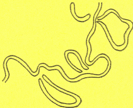
Oxbow lakes along the Mississippi River in Aitkin County. These are abandoned meander loops of the river.
